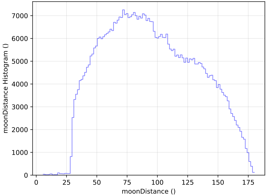
too_elab_heavy_r64_d2_gz_v3.4_10yrs WFD i band: moonDistance Histogram
