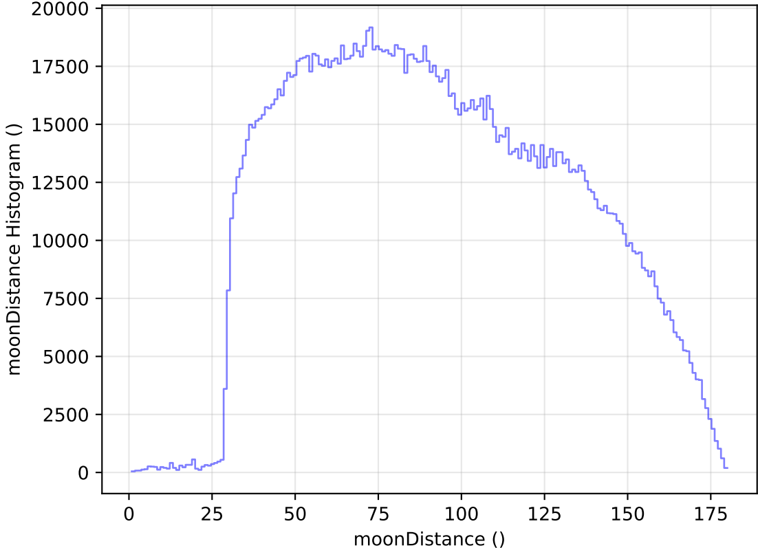
too_elab_heavy_r64_d2_gz_v3.4_10yrs WFD all bands: moonDistance Histogram
