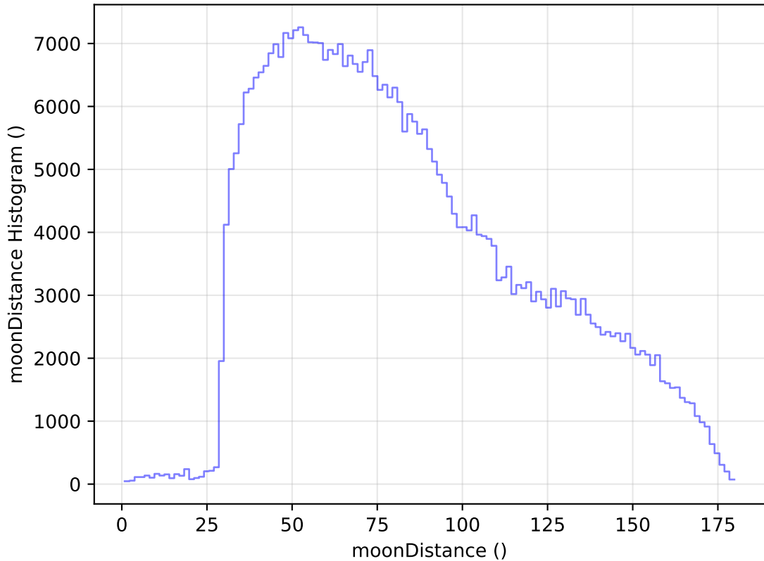
too_elab_heavy_r64_d2_gz_v3.4_10yrs All sky z band: moonDistance Histogram
