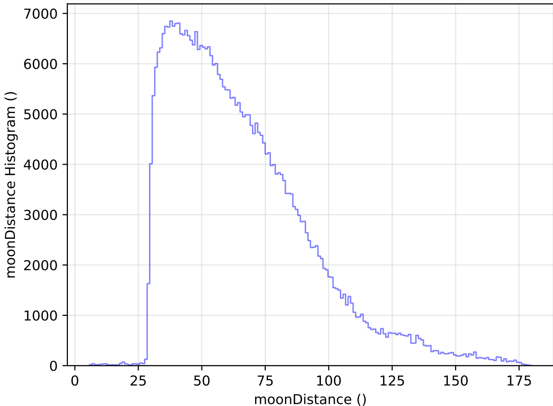
too_elab_heavy_r64_d2_gz_v3.4_10yrs All sky y band: moonDistance Histogram
