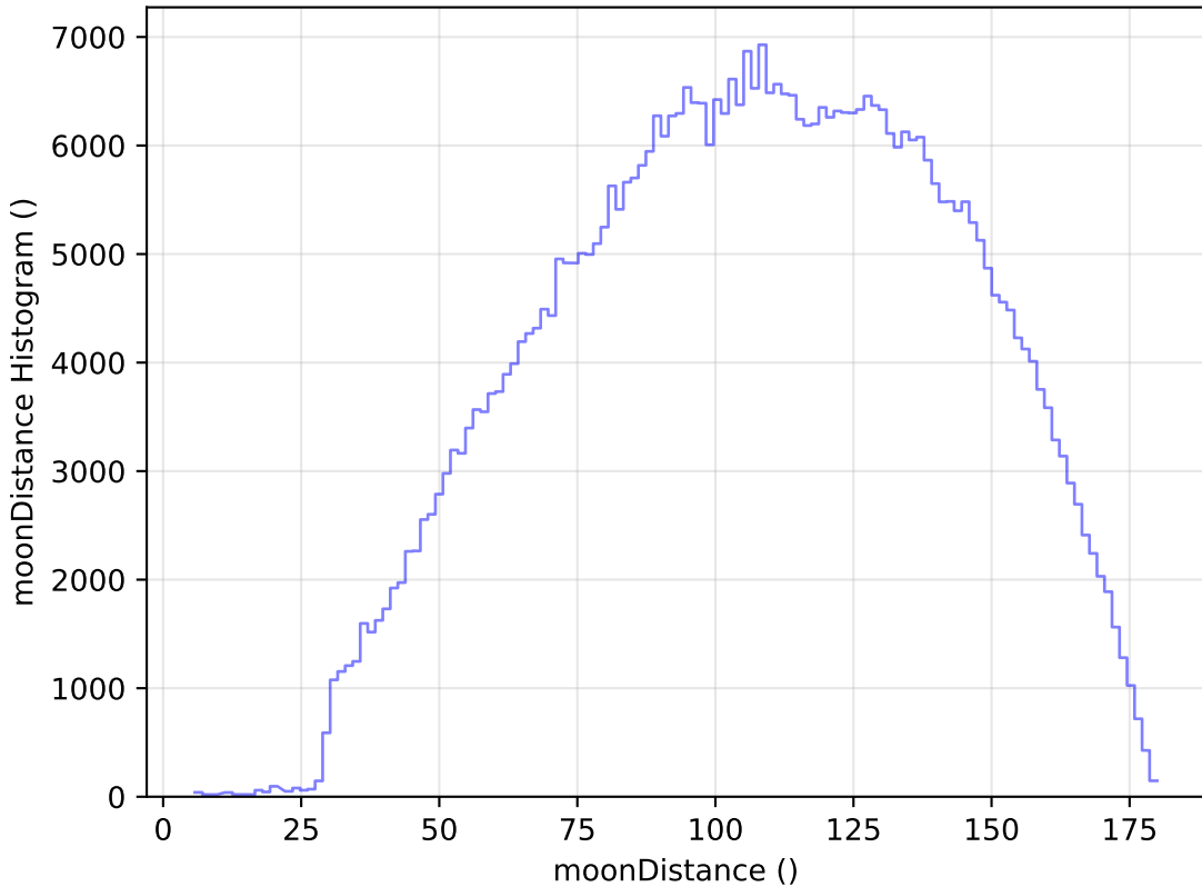
too_elab_heavy_r64_d2_gz_v3.4_10yrs All sky r band: moonDistance Histogram
