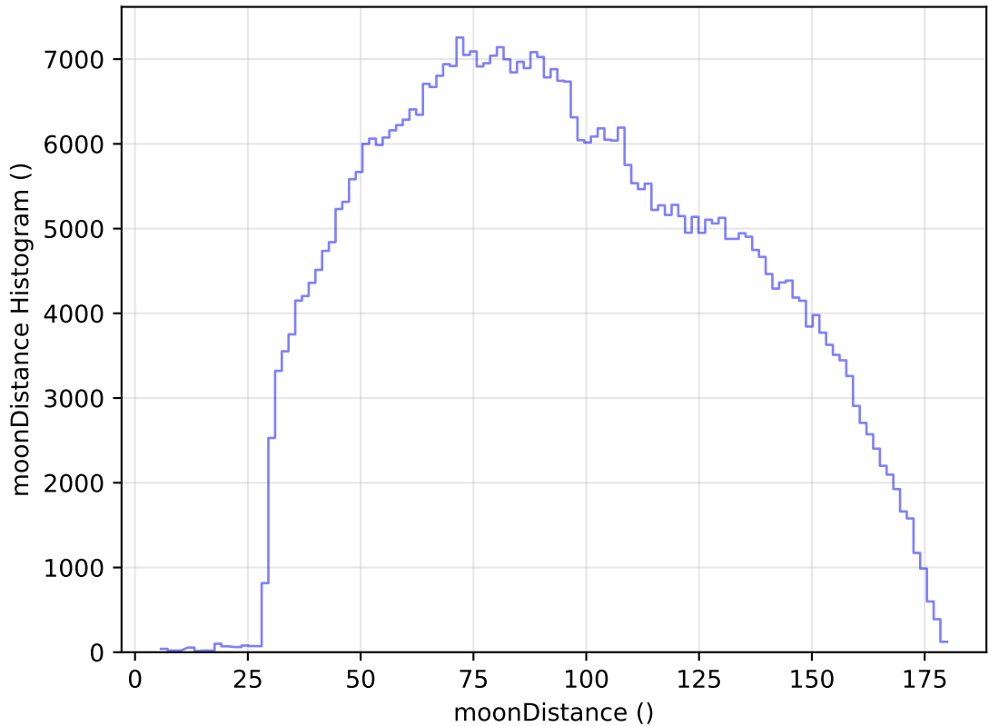
too_elab_heavy_r64_d2_gz_v3.4_10yrs All sky i band: moonDistance Histogram
