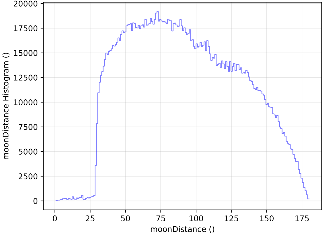
too_elab_heavy_r64_d2_gz_v3.4_10yrs All sky all bands: moonDistance Histogram
