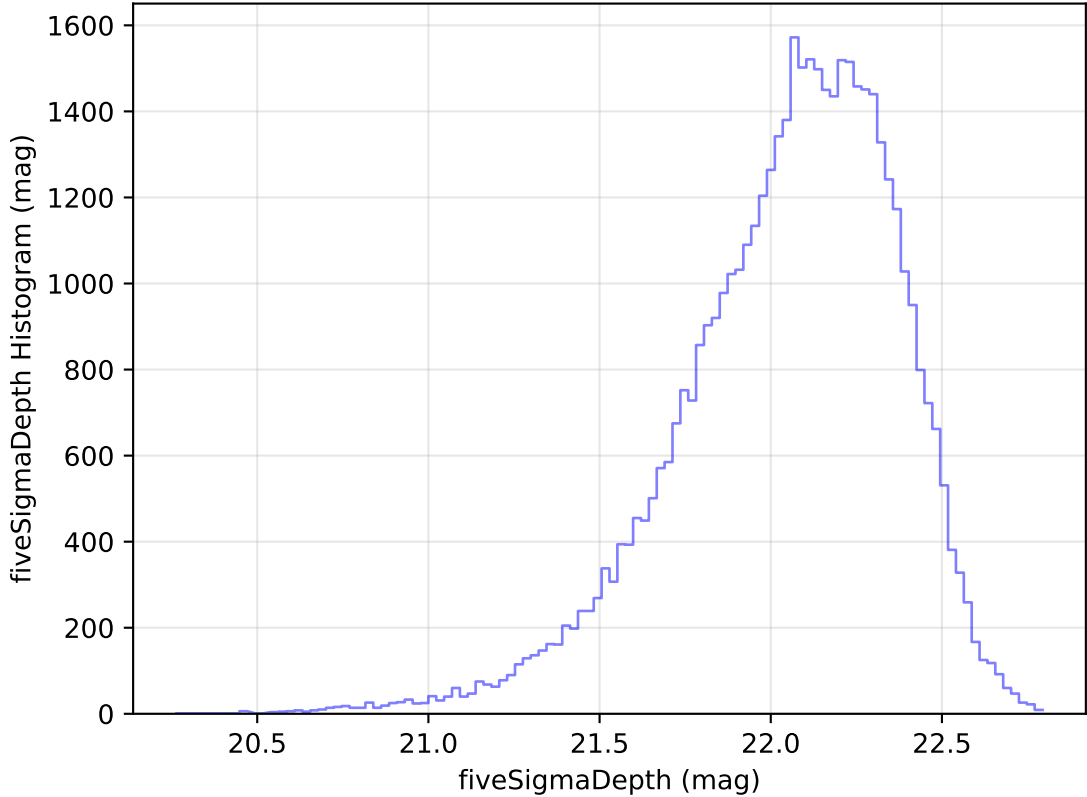
too_elab_heavy_r64_d2_gz_v3.4_10yrs Yr 1 y band: fiveSigmaDepth Histogram
