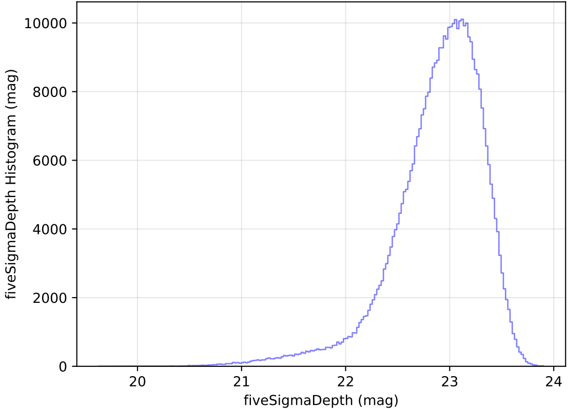
too_elab_heavy_r64_d2_gz_v3.4_10yrs WFD z band: fiveSigmaDepth Histogram
