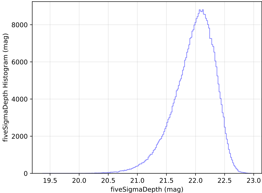
too_elab_heavy_r64_d2_gz_v3.4_10yrs WFD y band: fiveSigmaDepth Histogram
