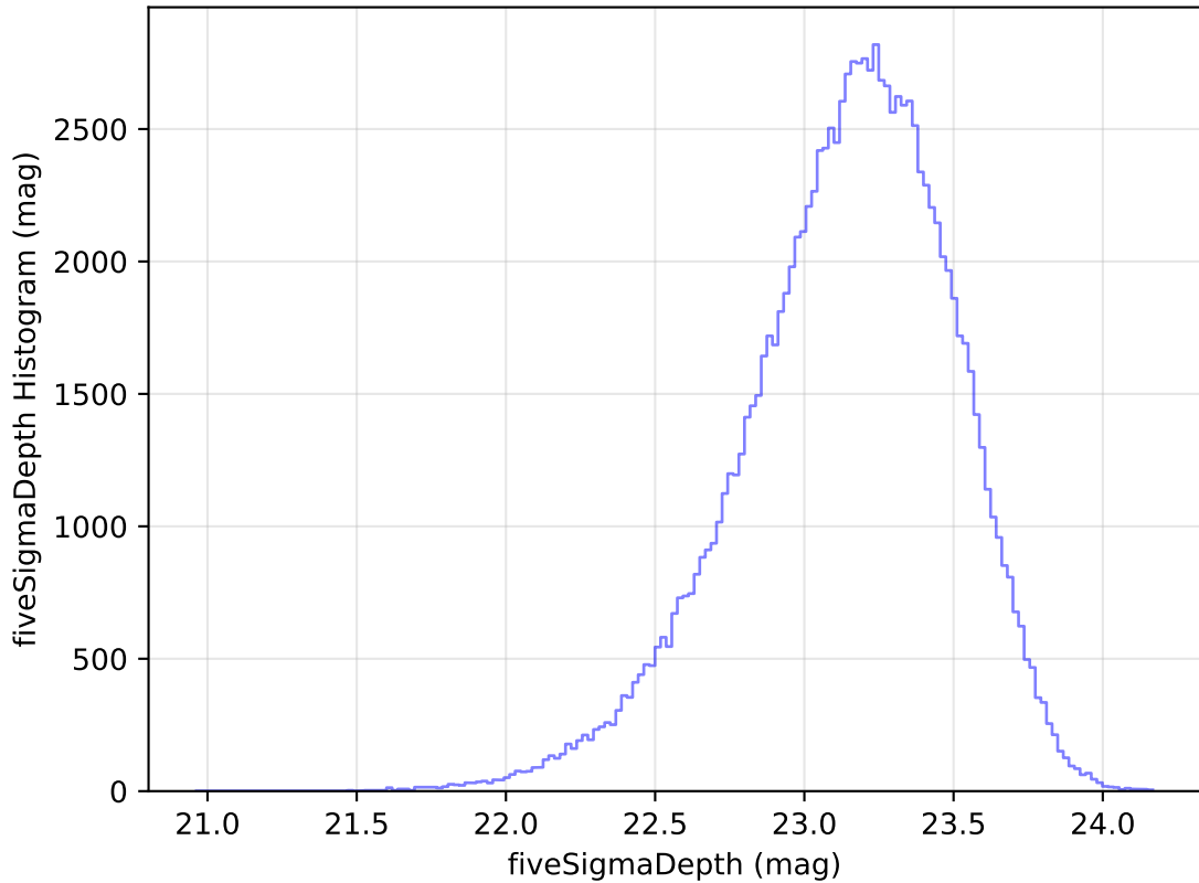
too_elab_heavy_r64_d2_gz_v3.4_10yrs WFD u band: fiveSigmaDepth Histogram
