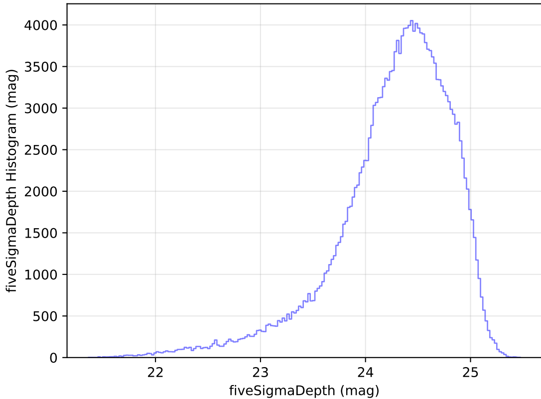
too_elab_heavy_r64_d2_gz_v3.4_10yrs WFD g band: fiveSigmaDepth Histogram
