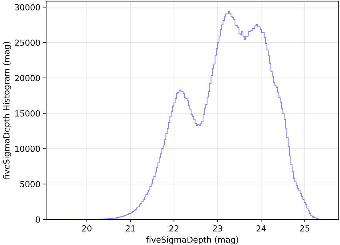
too_elab_heavy_r64_d2_gz_v3.4_10yrs WFD all bands: fiveSigmaDepth Histogram
