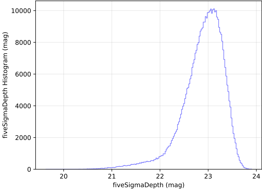
too_elab_heavy_r64_d2_gz_v3.4_10yrs All sky z band: fiveSigmaDepth Histogram
