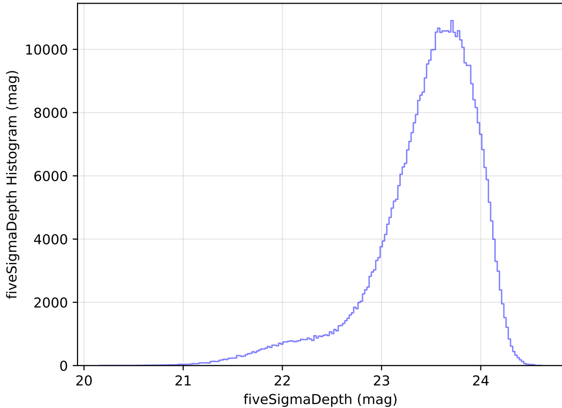
too_elab_heavy_r64_d2_gz_v3.4_10yrs All sky i band: fiveSigmaDepth Histogram
