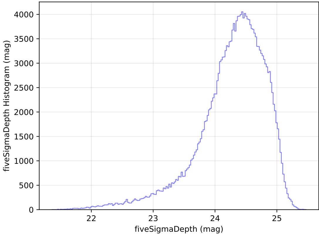
too_elab_heavy_r64_d2_gz_v3.4_10yrs All sky g band: fiveSigmaDepth Histogram
