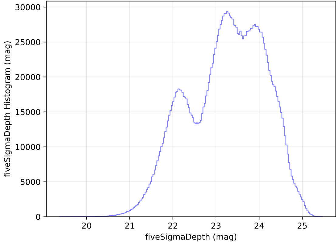
too_elab_heavy_r64_d2_gz_v3.4_10yrs All sky all bands: fiveSigmaDepth Histogram
