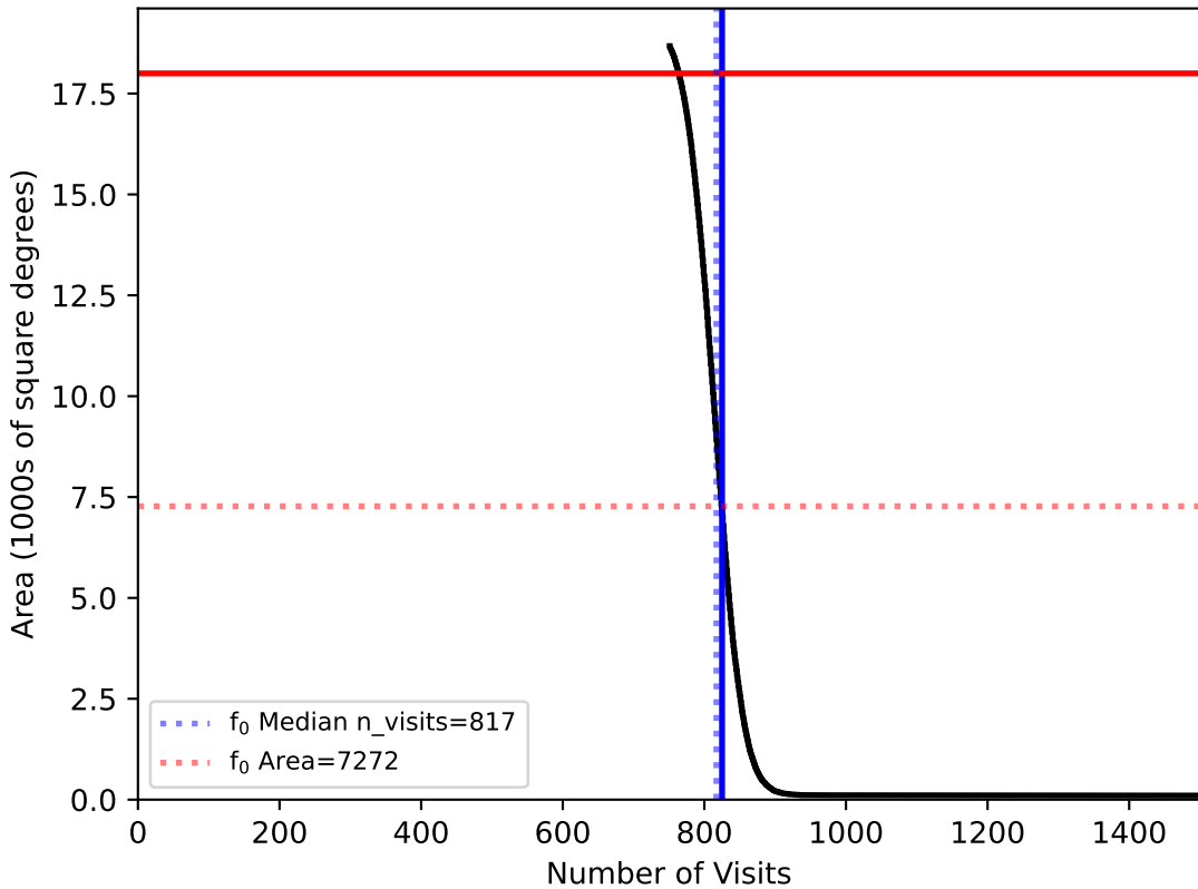
too_elab_heavy_r64_d2_gz_v3.4_10yrs WFD: f0
