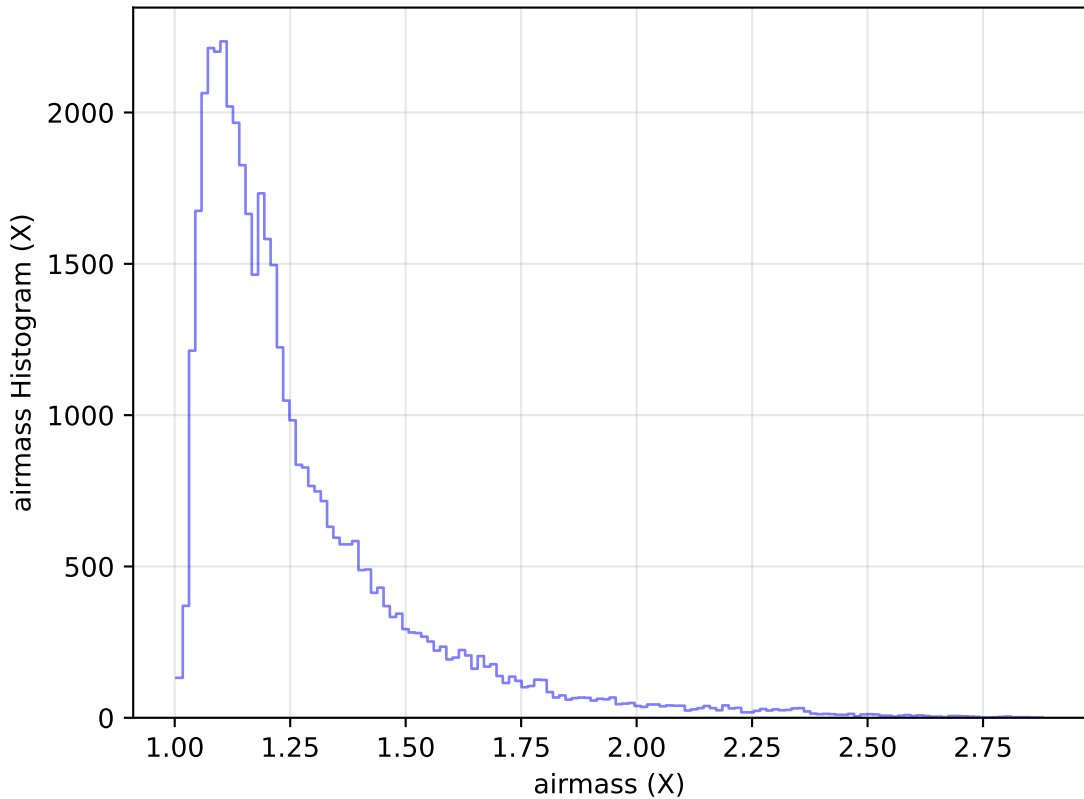
too_elab_heavy_r64_d2_gz_v3.4_10yrs Yr 1 z band: airmass Histogram
