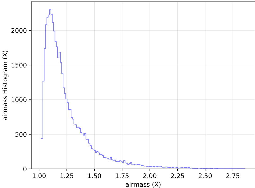
too_elab_heavy_r64_d2_gz_v3.4_10yrs Yr 1 y band: airmass Histogram
