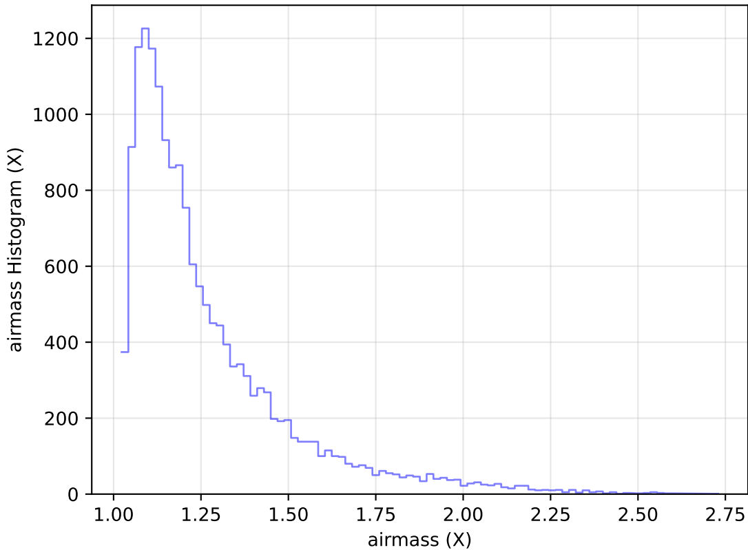
too_elab_heavy_r64_d2_gz_v3.4_10yrs Yr 1 u band: airmass Histogram
