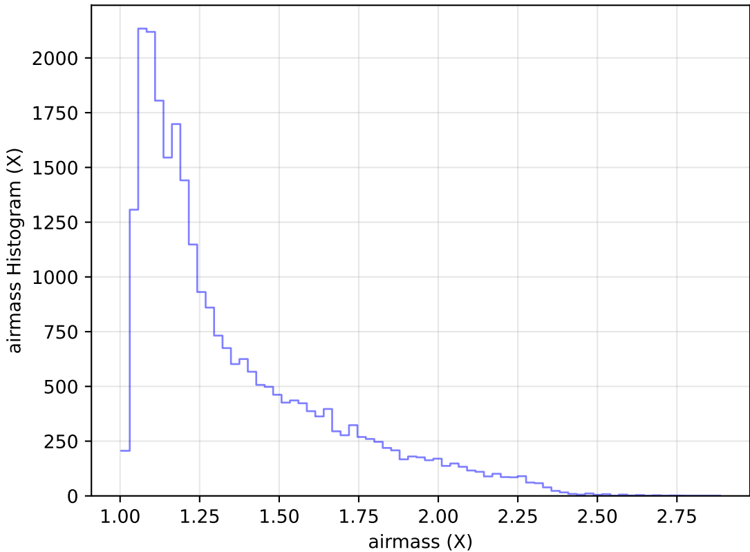
too_elab_heavy_r64_d2_gz_v3.4_10yrs Yr 1 g band: airmass Histogram
