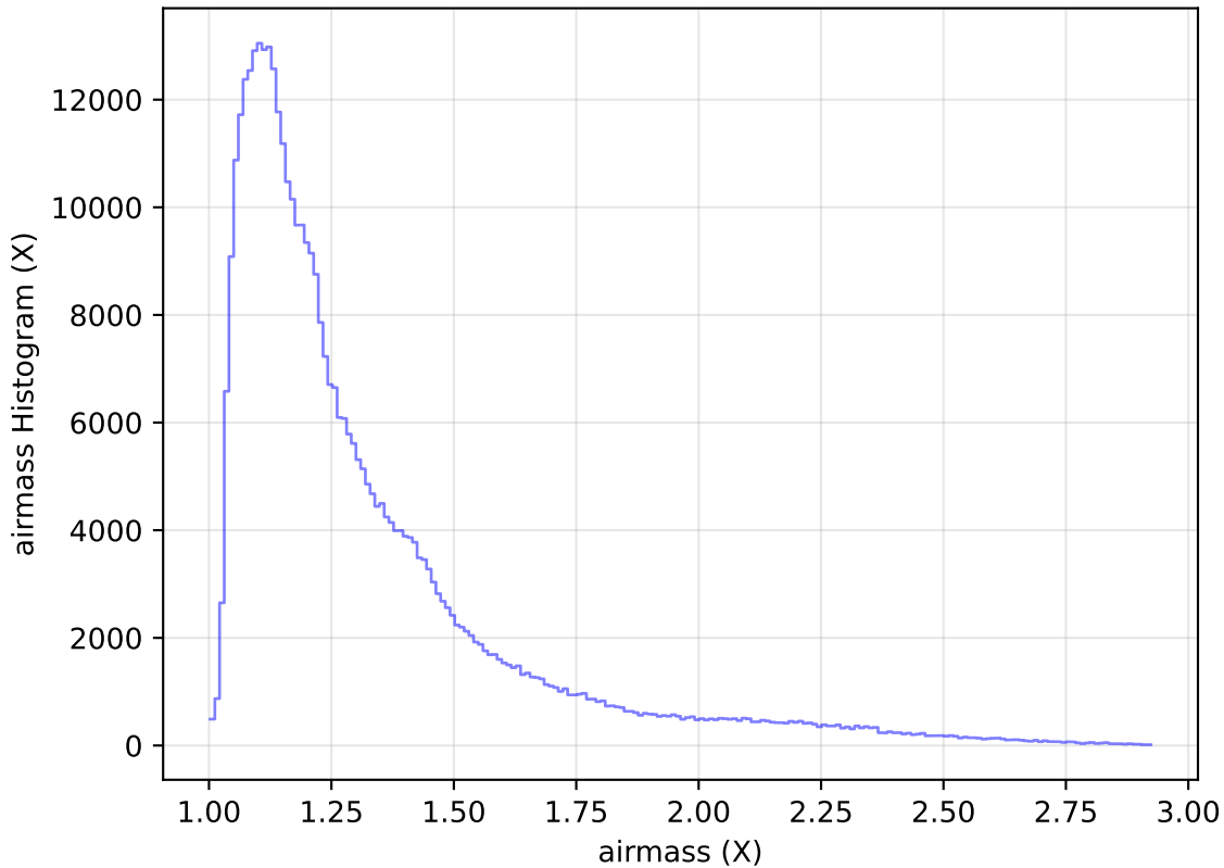
too_elab_heavy_r64_d2_gz_v3.4_10yrs WFD z band: airmass Histogram
