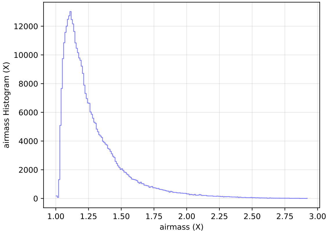
too_elab_heavy_r64_d2_gz_v3.4_10yrs WFD y band: airmass Histogram
