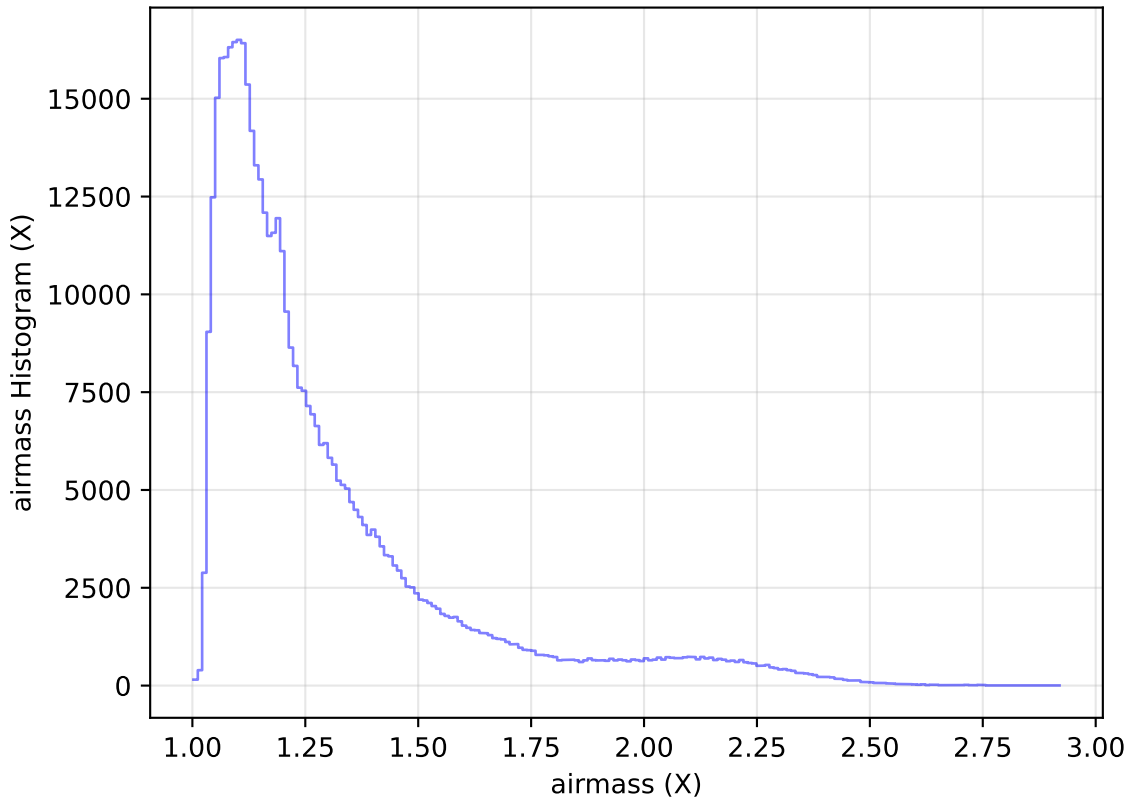
too_elab_heavy_r64_d2_gz_v3.4_10yrs WFD r band: airmass Histogram
