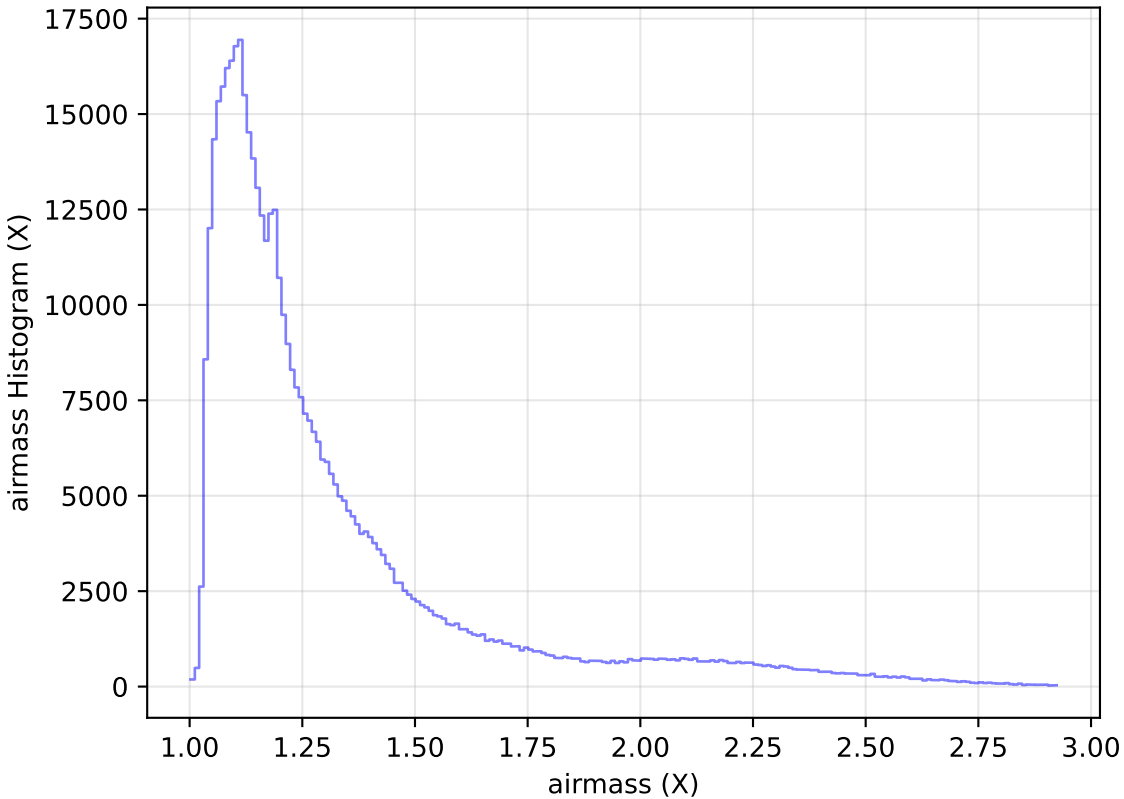
too_elab_heavy_r64_d2_gz_v3.4_10yrs WFD i band: airmass Histogram
