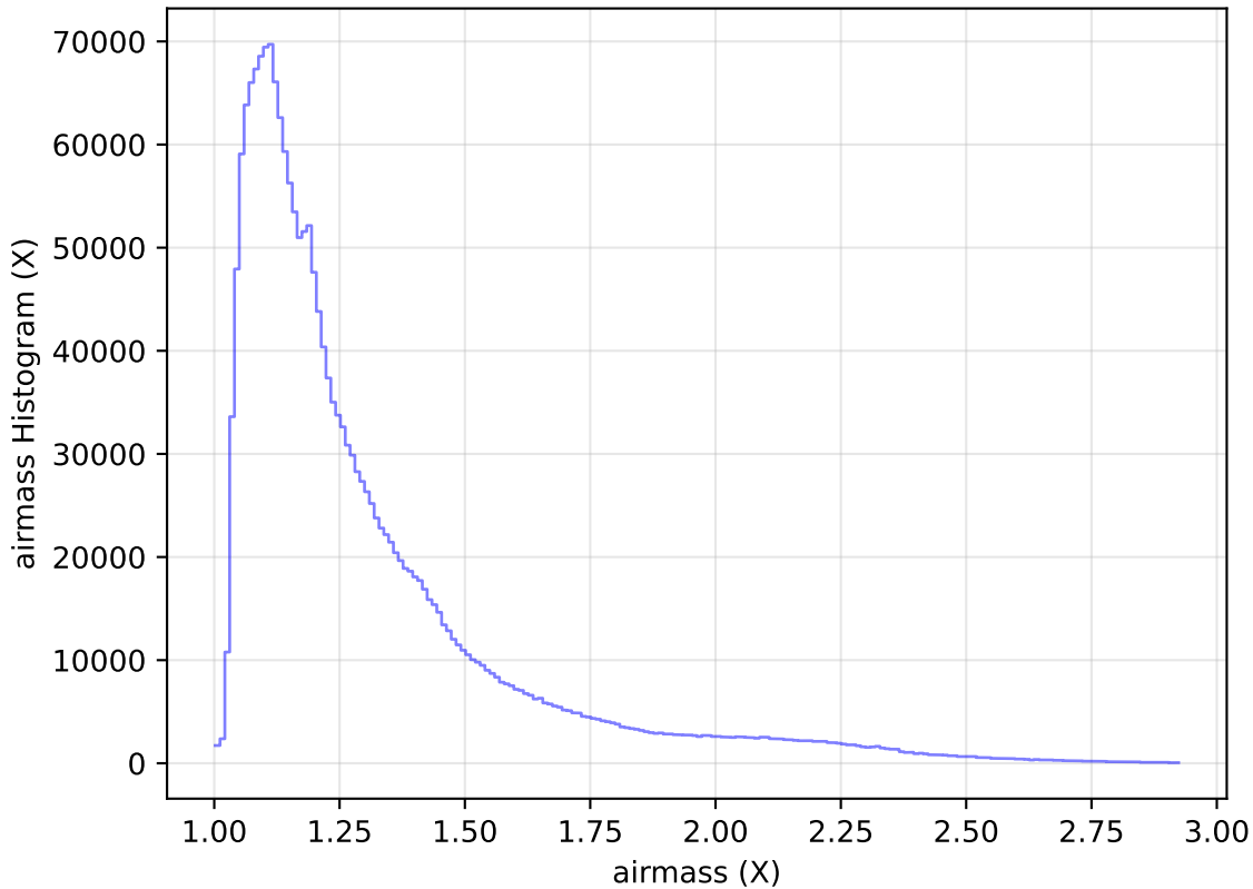
too_elab_heavy_r64_d2_gz_v3.4_10yrs WFD all bands: airmass Histogram
