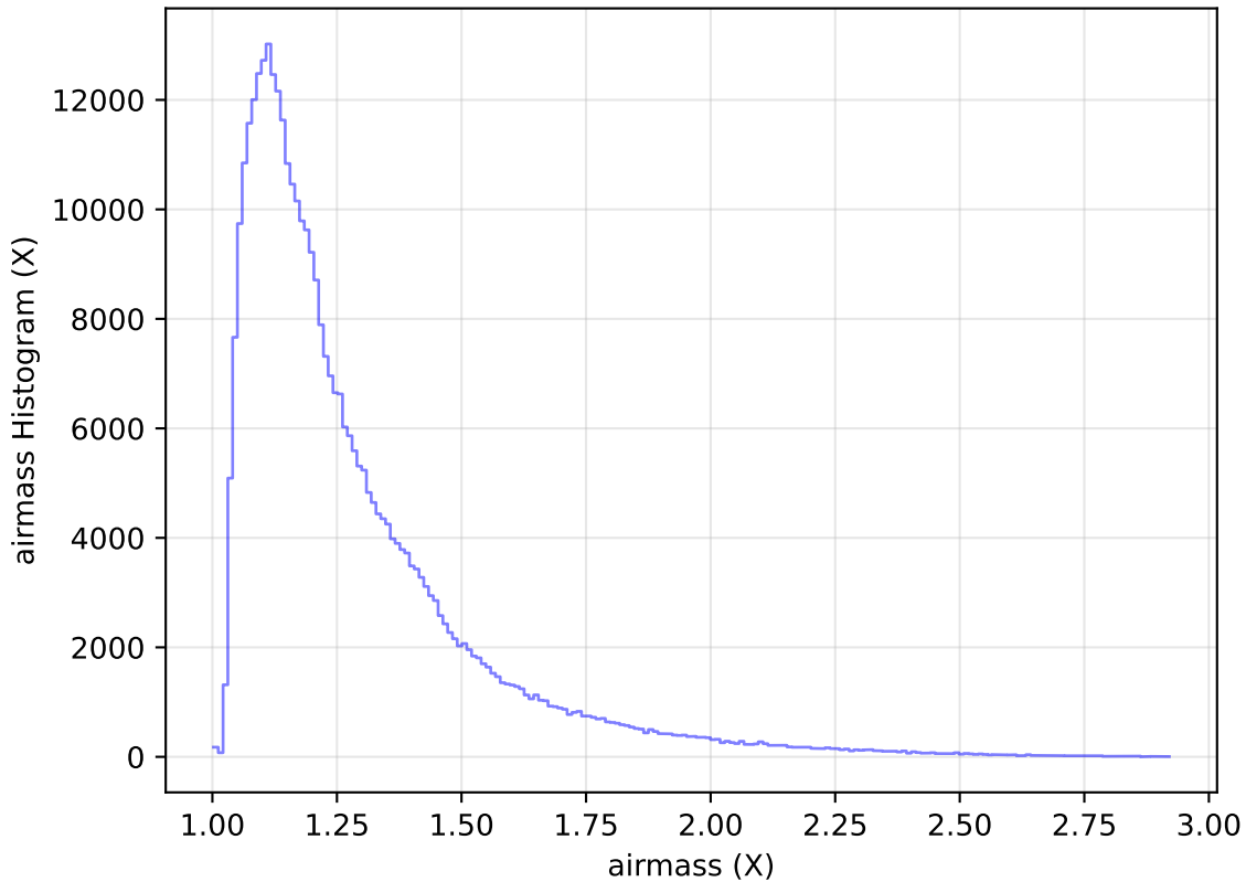
too_elab_heavy_r64_d2_gz_v3.4_10yrs All sky y band: airmass Histogram
