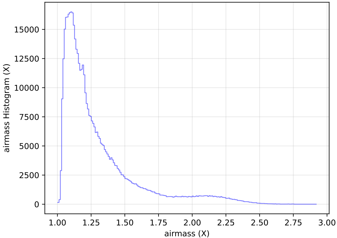
too_elab_heavy_r64_d2_gz_v3.4_10yrs All sky r band: airmass Histogram
