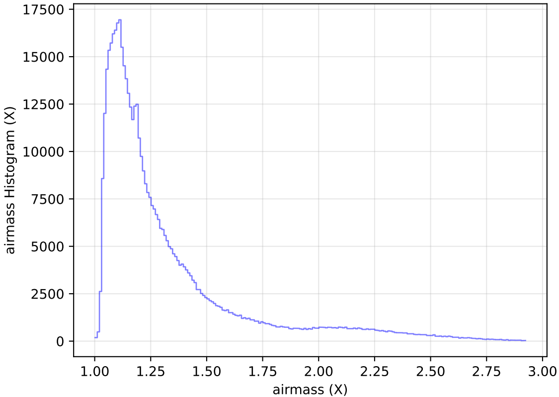
too_elab_heavy_r64_d2_gz_v3.4_10yrs All sky i band: airmass Histogram
