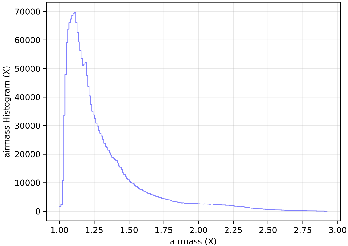
too_elab_heavy_r64_d2_gz_v3.4_10yrs All sky all bands: airmass Histogram
