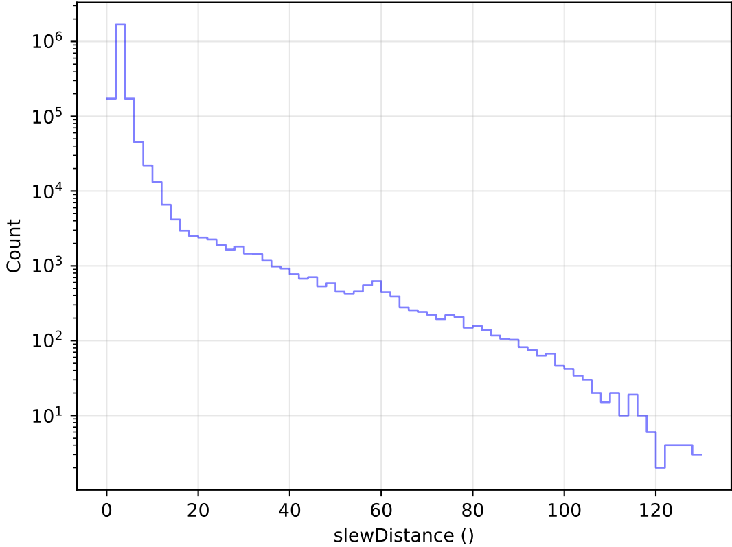
too_elab_heavy_r64_d2_gz_v3.4_10yrs All visits: Slew Distance Histogram
