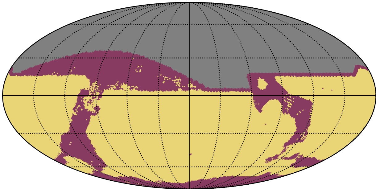
too_elab_heavy_r64_d2_gz_v3.4_10yrs All sky: RapidRevisits
