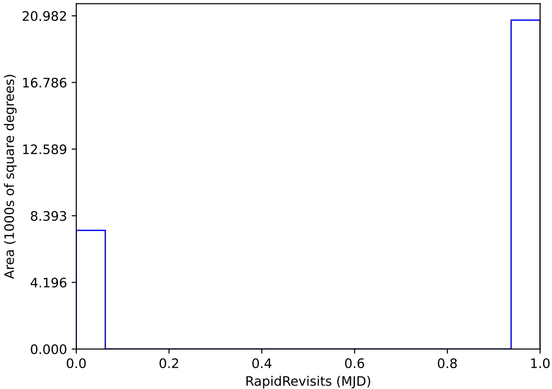
too_elab_heavy_r64_d2_gz_v3.4_10yrs All sky: RapidRevisits
