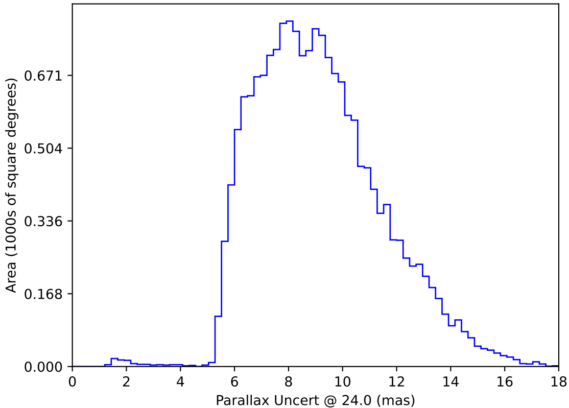
too_elab_heavy_r64_d2_gz_v3.4_10yrs WFD: Parallax Uncert @ 24.0
