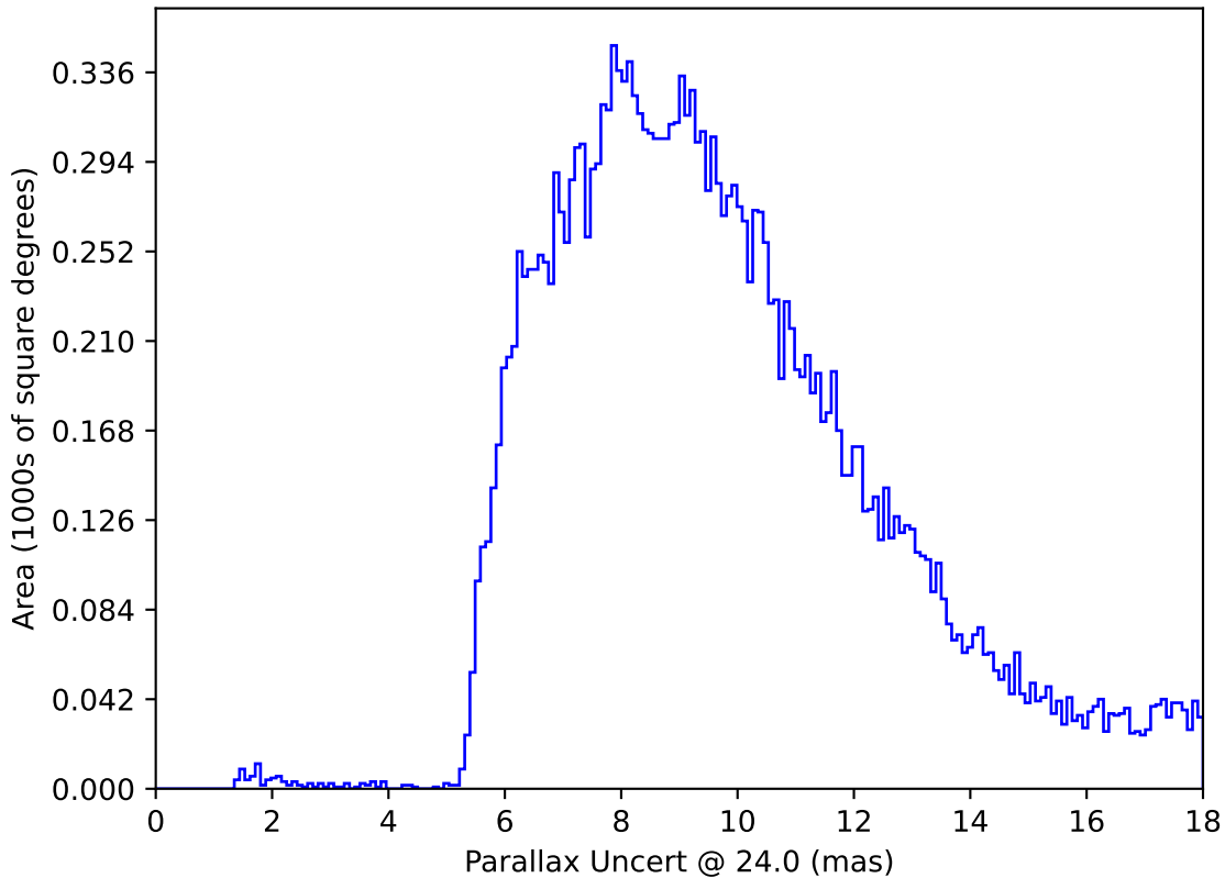
too_elab_heavy_r64_d2_gz_v3.4_10yrs All sky: Parallax Uncert @ 24.0
