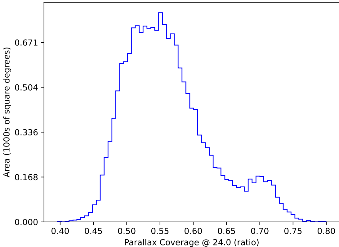
too_elab_heavy_r64_d2_gz_v3.4_10yrs WFD: Parallax Coverage @ 24.0
