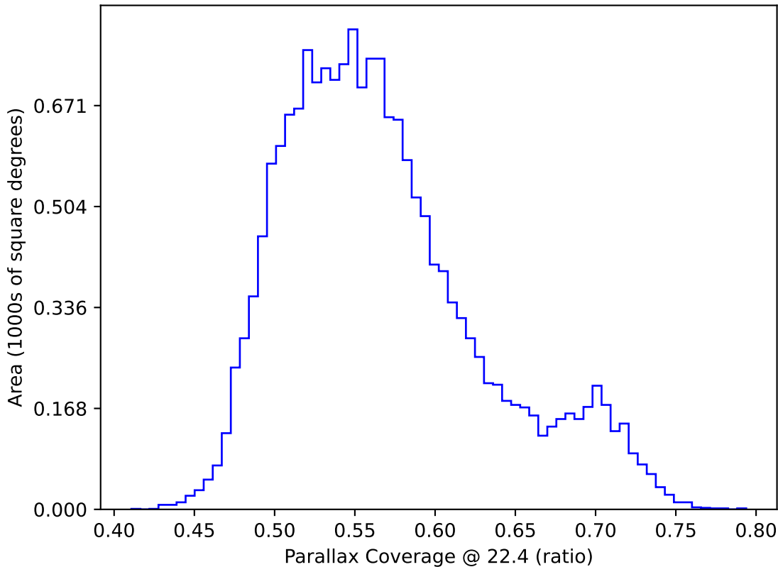
too_elab_heavy_r64_d2_gz_v3.4_10yrs WFD: Parallax Coverage @ 22.4
