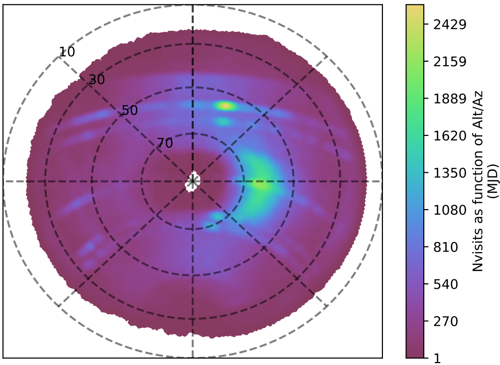
too_elab_heavy_r64_d2_gz_v3.4_10yrs z band: Nvisits as function of Alt/Az
