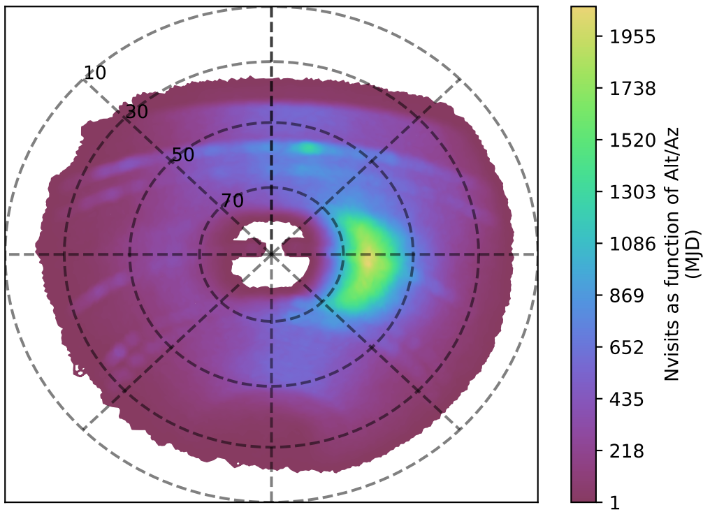
too_elab_heavy_r64_d2_gz_v3.4_10yrs y band: Nvisits as function of Alt/Az
