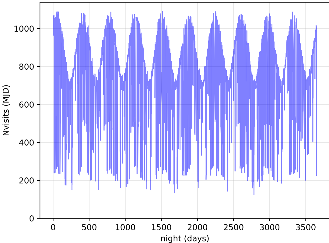
too_elab_heavy_r64_d2_gz_v3.4_10yrs All visits: Nvisits
