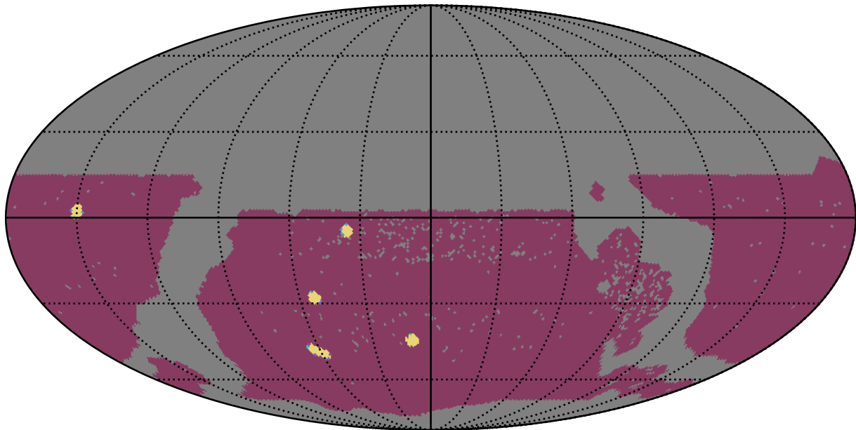
too_elab_heavy_r64_d2_gz_v3.4_10yrs WFD: NumberOfQuickRevisits
