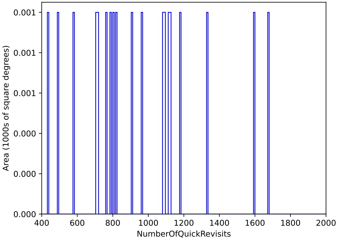
too_elab_heavy_r64_d2_gz_v3.4_10yrs WFD: NumberOfQuickRevisits
