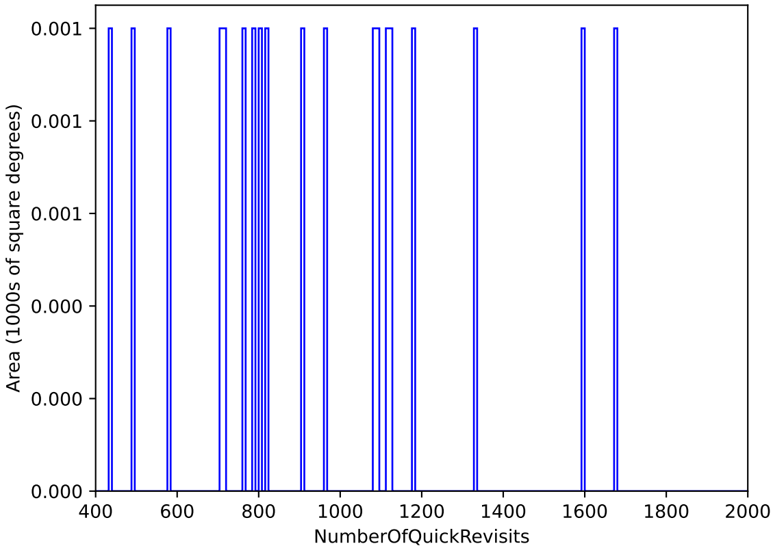
too_elab_heavy_r64_d2_gz_v3.4_10yrs All sky: NumberOfQuickRevisits
