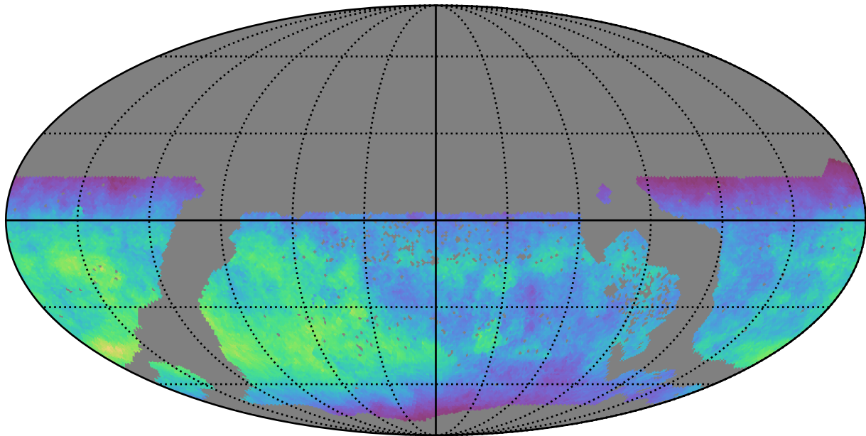
too_elab_heavy_r64_d2_gz_v3.4_10yrs WFD z band: Normalized Teff
