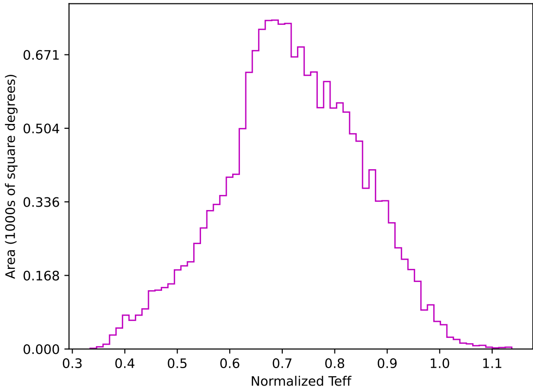
too_elab_heavy_r64_d2_gz_v3.4_10yrs WFD z band: Normalized Teff
