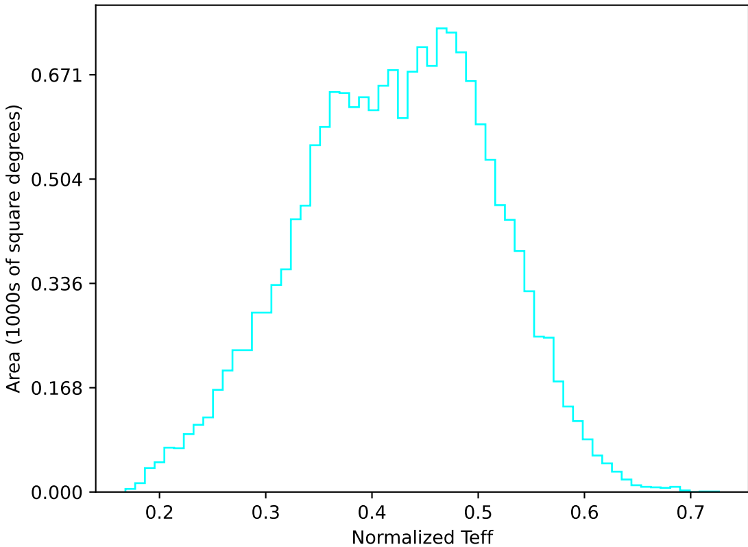
too_elab_heavy_r64_d2_gz_v3.4_10yrs WFD u band: Normalized Teff
