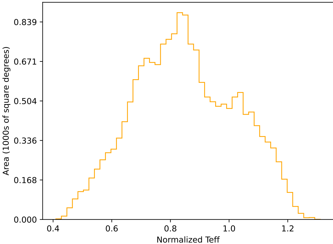
too_elab_heavy_r64_d2_gz_v3.4_10yrs WFD r band: Normalized Teff
