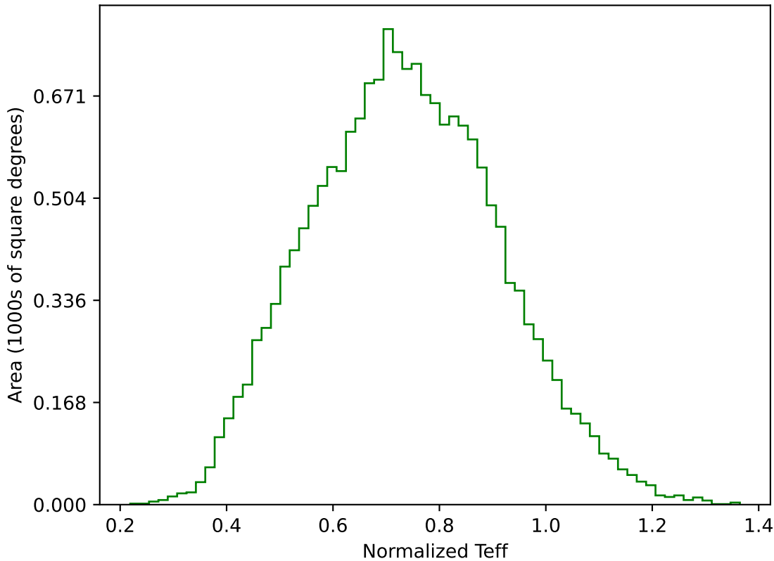
too_elab_heavy_r64_d2_gz_v3.4_10yrs WFD g band: Normalized Teff
