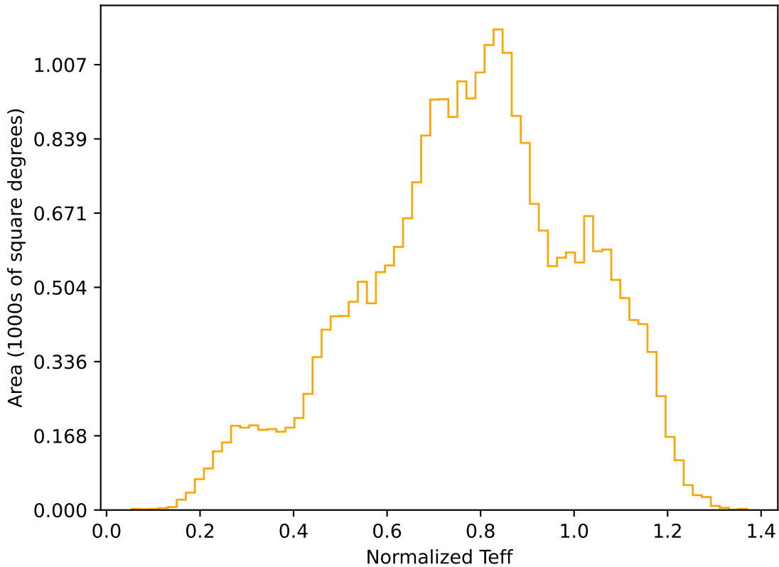
too_elab_heavy_r64_d2_gz_v3.4_10yrs All sky r band: Normalized Teff
